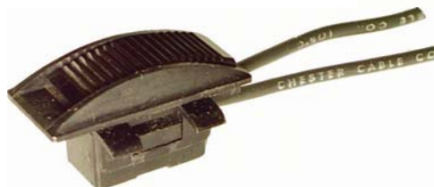
81805A SPST ON - OFF 6 amp. 125 VAC
