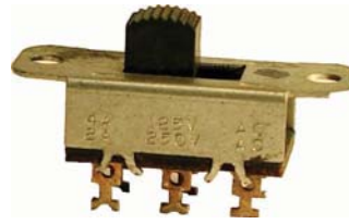
18-139 DPDT ON - ON 4 amp. 125 VAC
