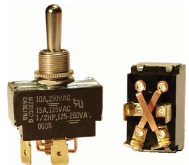
6G053 DPDT MOM. ON - OFF - MOM. ON 15 amp. 125 volt
