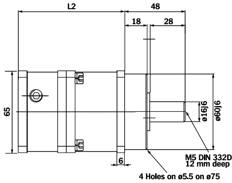
GBSM80-MNT080-XX
