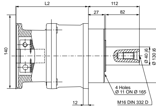
GBSM100-MNT180-XX
